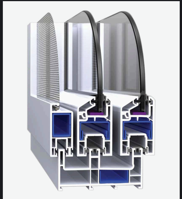
I-60 sliding reference cutaway.
