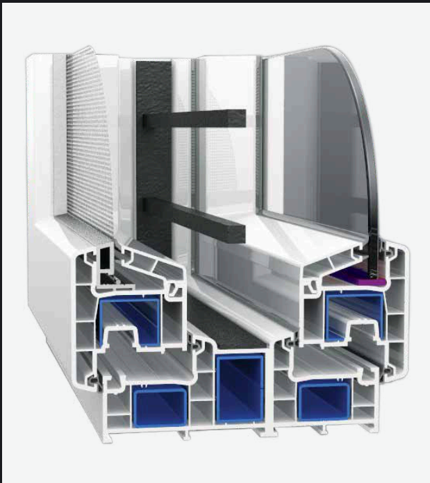
I-60 casement reference cutaway.
